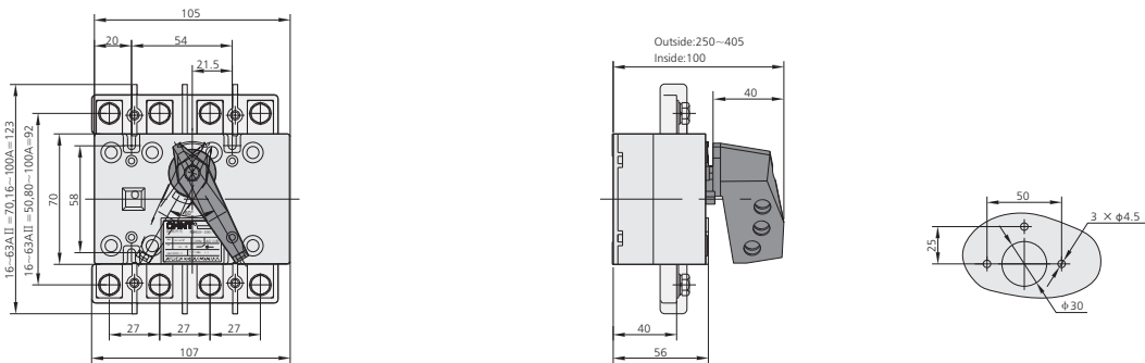
Mounting dimension of externally mounted handle
