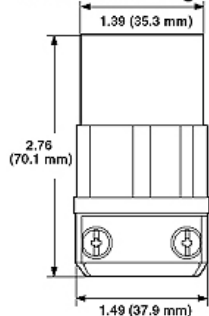
Dimensional Diagram
