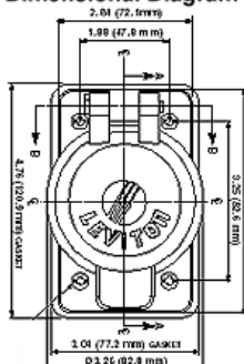
Dimensional Diagram
