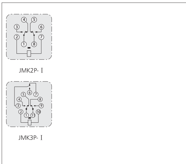
Internal connection (bottom view)
