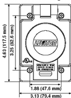
Dimensional Diagram
