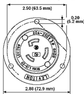
Dimensional Diagram
