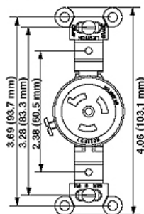
Dimensional Diagram
